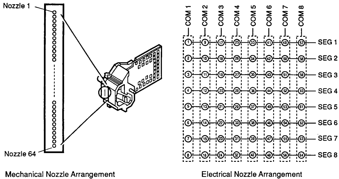
Figure 1-4 Nozzle Arrangement
