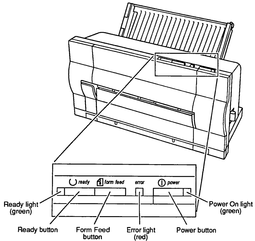
Figure 1-12 Operation Panel
