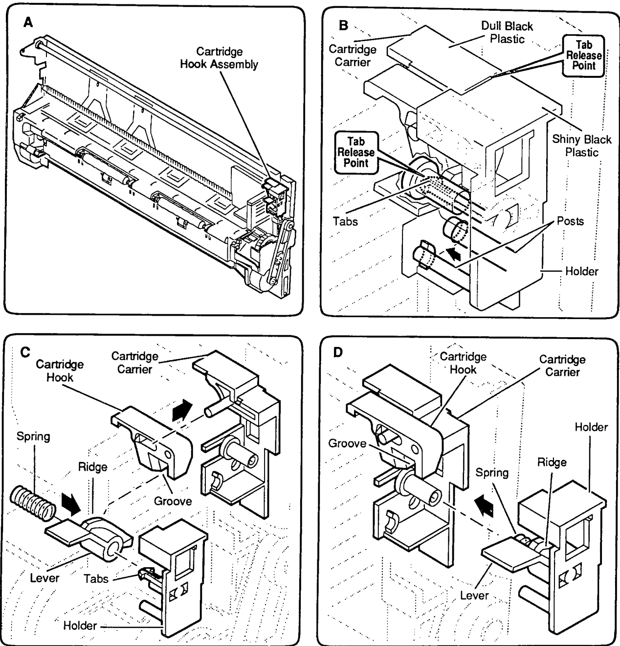
Figure 2-6 Cartridge Hook
