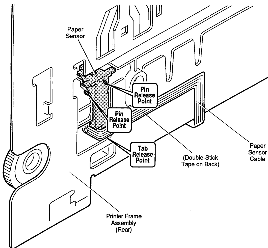
Figure 2-8 Paper Sensor
