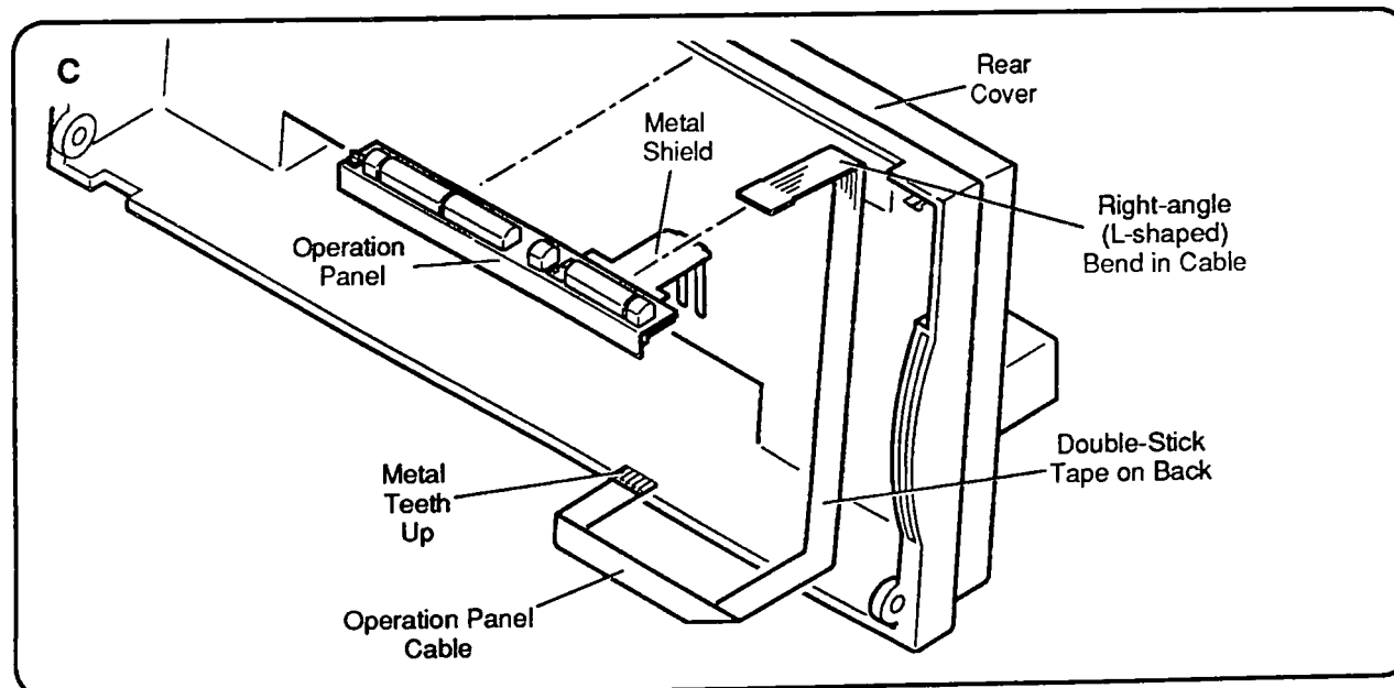
Figure 2-5 Operation Panel Assembly and Cable
