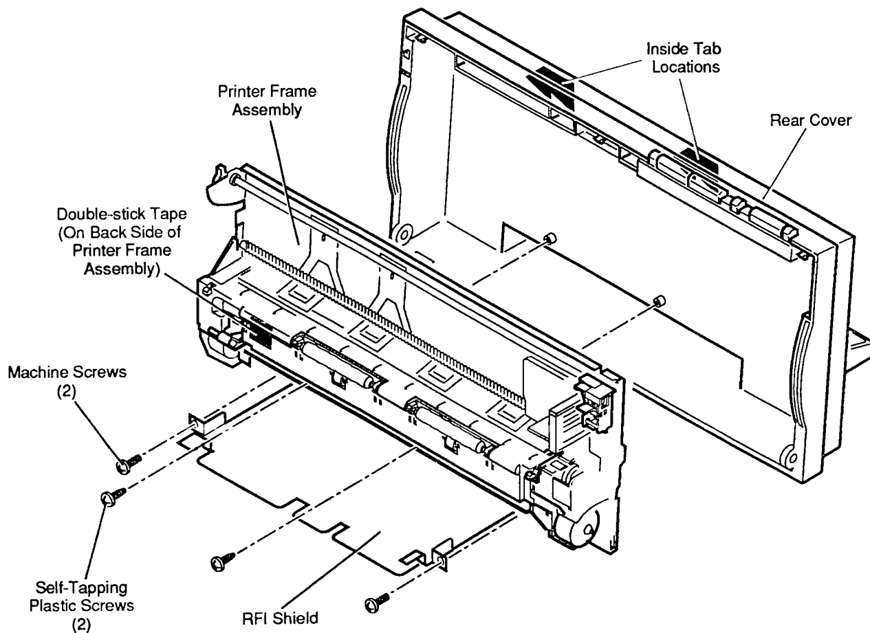
Figure 2-4 Printer Frame Assembly
