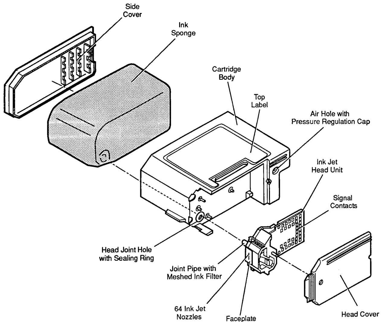
Figure 1-2 Ink Cartridge Structure
