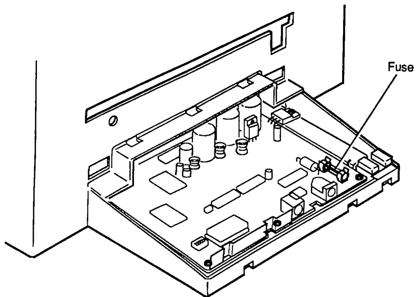
Figure 2-11 Fuse
