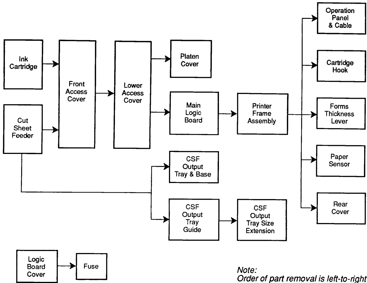
StyleWriter Take-Apart Flowchart
