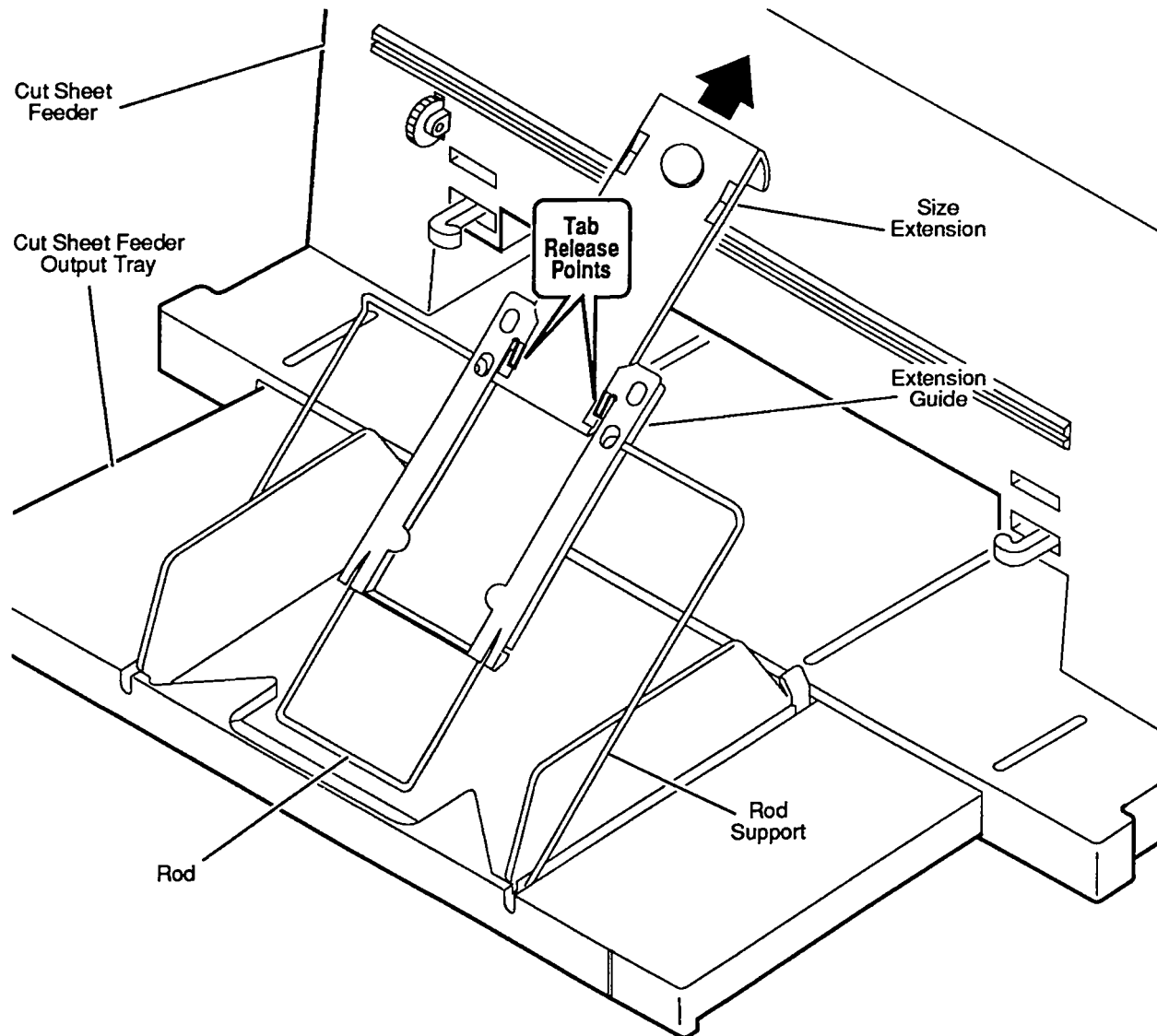
Figure 2-12 Output Tray Size Extension
