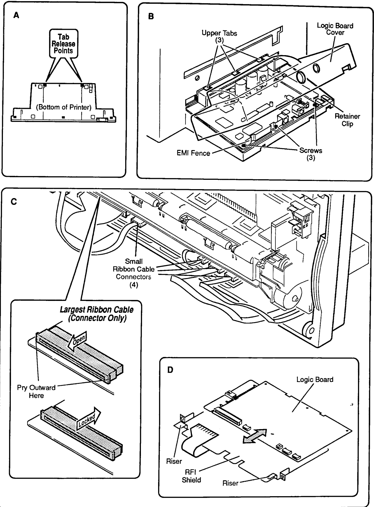
Figure 2-3 Main Logic Board
