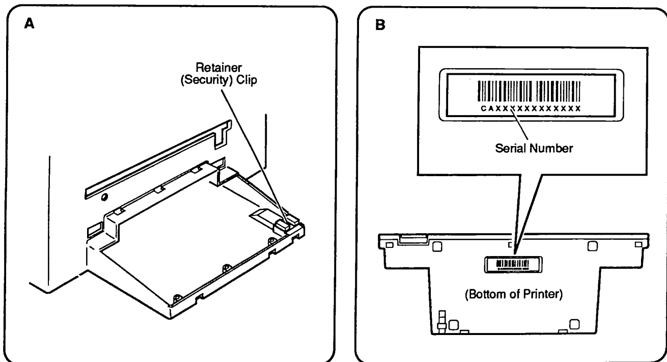
Figure 2-10 Rear Cover
