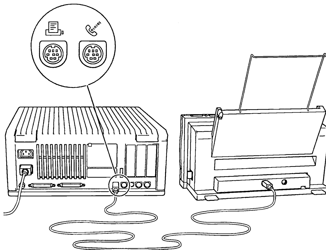
Figure 1-6 Making the Serial Connection
