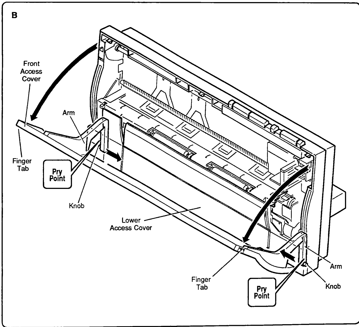
Figure 2-1 Front Access Cover
