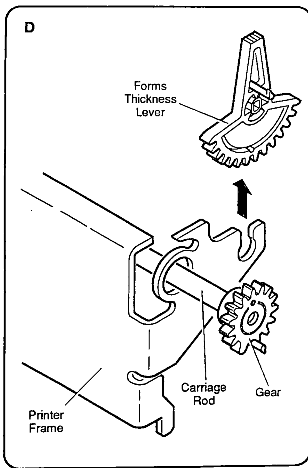
Figure 2-7 Forms Thickness Lever
