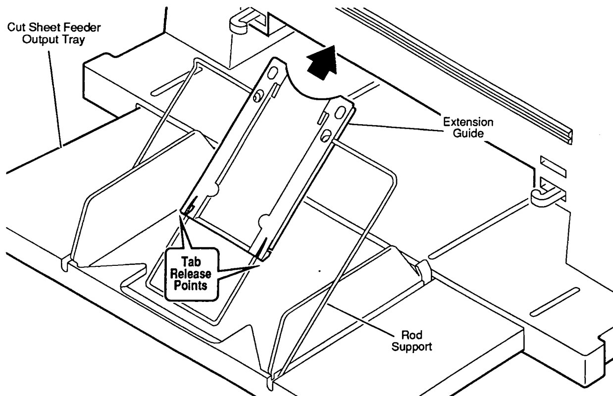
Figure 2-13 Output Tray Extension Guide
