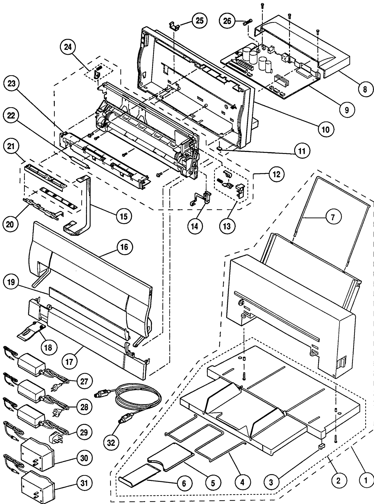
Figure 1 Exploded View
