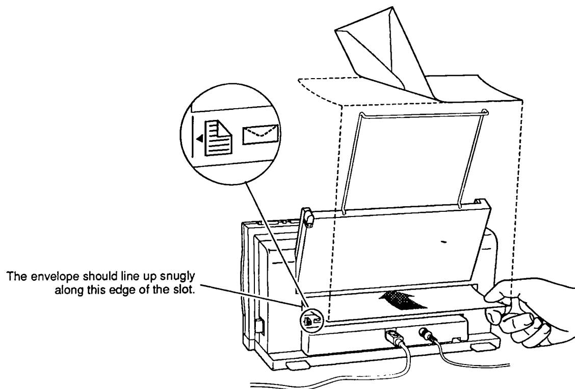
Figure 1-11 Manual Feed (Rear Slot)
