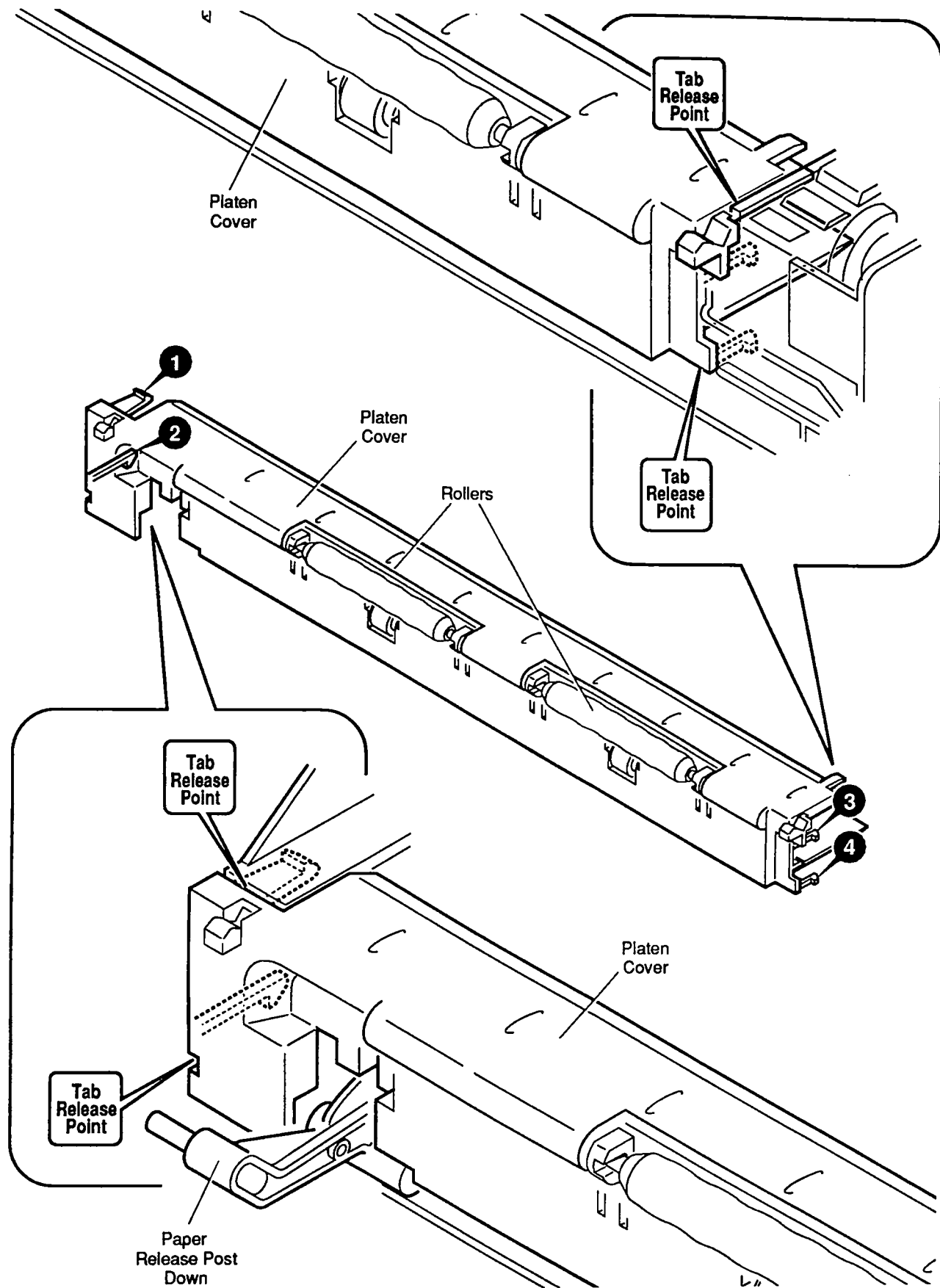
Figure 2-9 Platen Cover and Rollers
