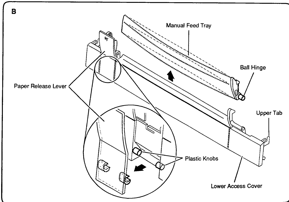
Figure 2-2 Lower Access Cover
