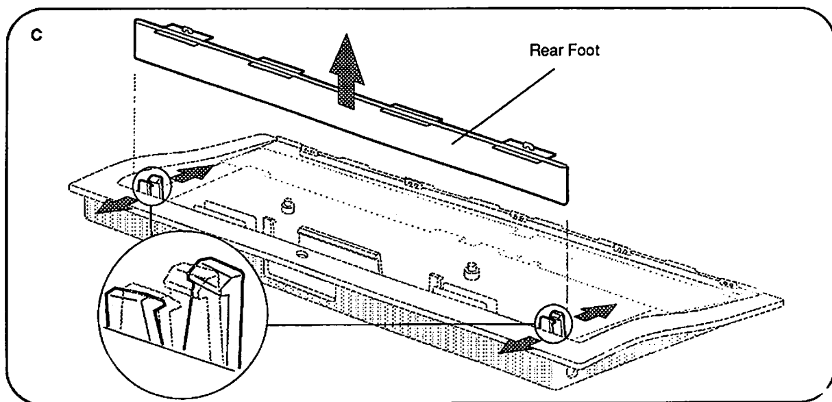
Figure 1-5 Adjustable Rear Foot and Foot Return Spring
